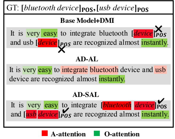
Figure 3: Visualization of attention for the \mathbb{R} \rightarrow \mathbb{L} pair.
